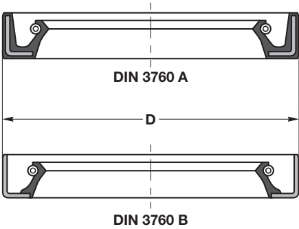
The press fit allowance and the eccentricity of oil seals are given in Table 874A .
